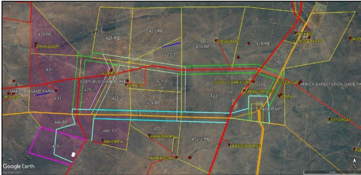
Figure 3.4: Proposed Makoppa PV grid connection assessment corridor alternatives: Alternative 1 Preferred (light blue), Alt 2 (green) and Alt 3 (white outline). Also indicated are the Tabor PV suite sites (pink shading), Makoppa PV site (pink outline), Makoppa substations (white fill), and properties affected by Alts 1-3 (yellow outlines), roads (red), existing Eskom transmission lines (orange), and landing strips (dark blue)
