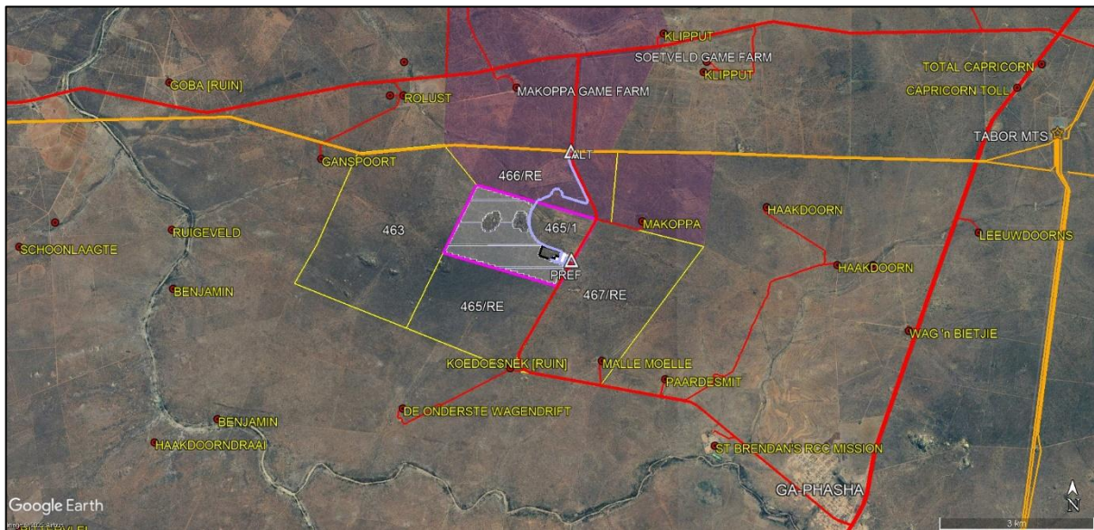
Figure 3.3: Makoppa PV site (pink outline) and adjacent properties (yellow outlines) in relation to proposed PV infrastructure: site access point alternatives (white triangles), project roads (grey), panel development areas (white shading), operational terrains (white outlines), and construction phase terrains (black outline). Also indicated are existing roads (red), existing Eskom transmission lines (orange), and other Tabor Solar PV Cluster sites (pink shading)
