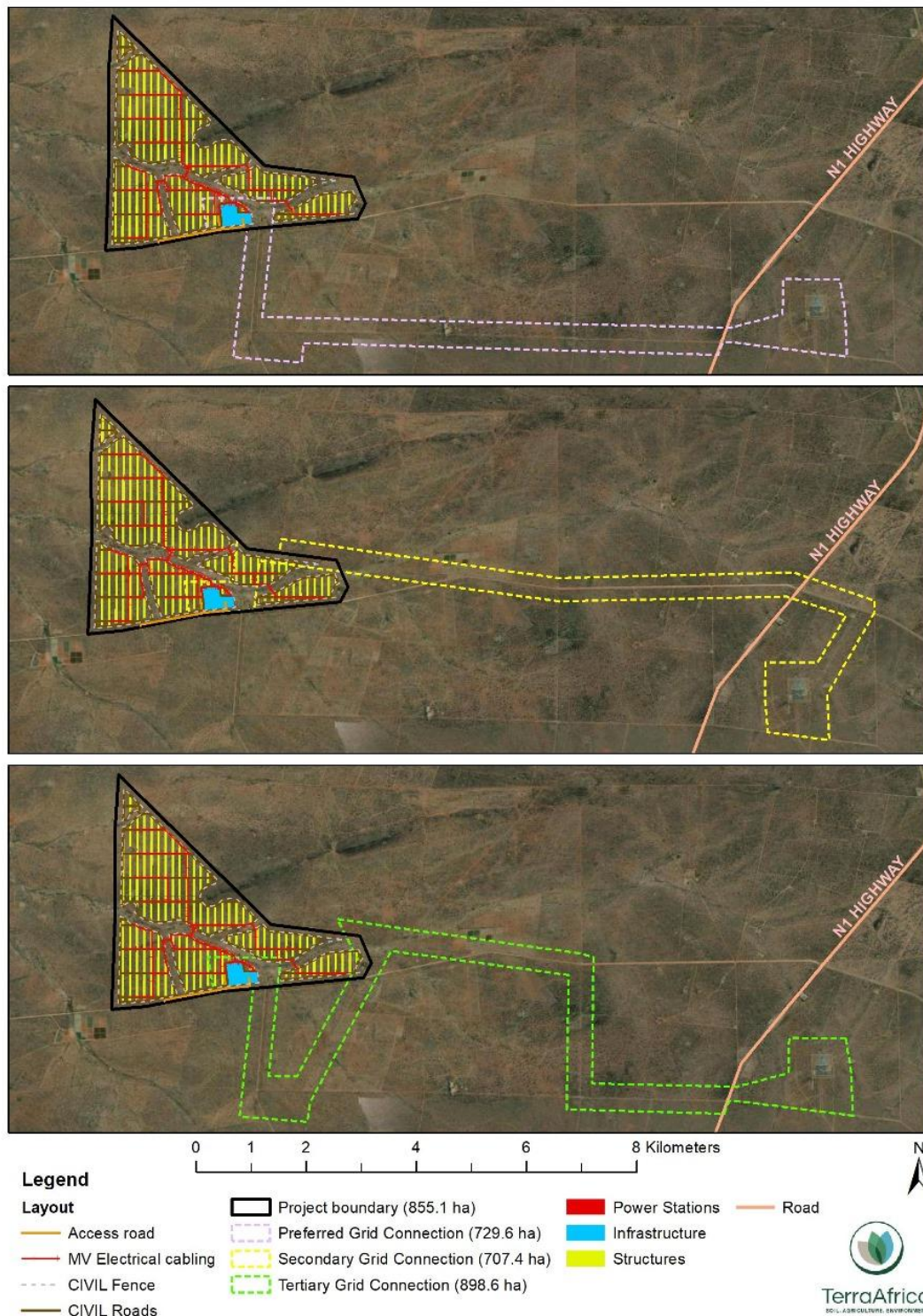
Figure 2: Layout map of the Draailoop Solar PV project and alternative locations of the grid connection corridor
