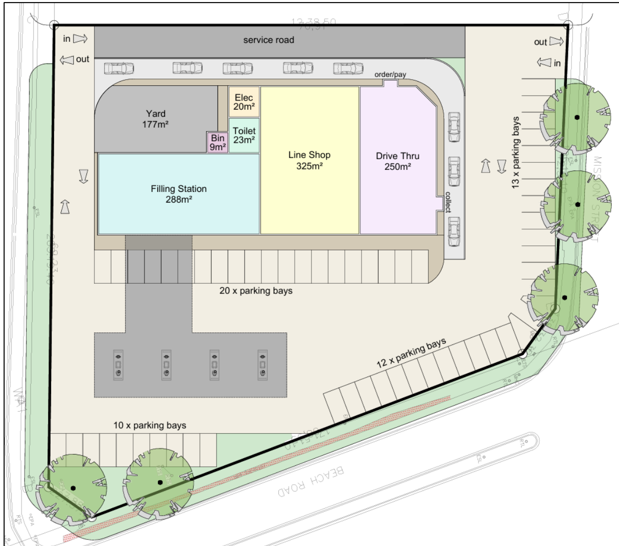
Figure 2: Site Development Plan of proposed filling station on Erf 7379, Pacaltsdorp (Gareths Calvert Designs t/a CCA, 2021).
