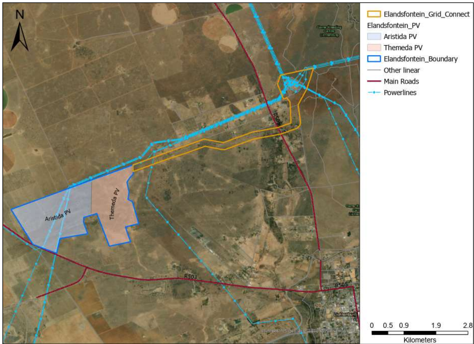
Figure 4: Proposed locality of the ElandsfonteinCluster and associated grid connection corridor.
