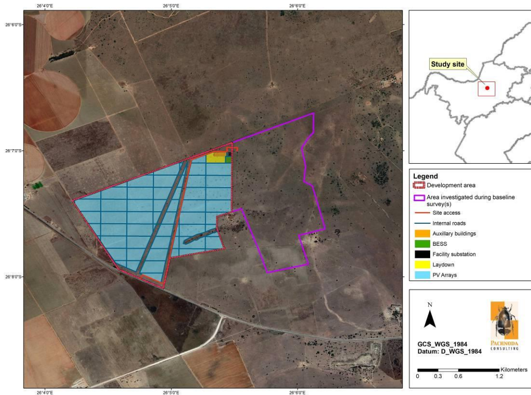
Figure 2: A satellite image illustrating the geographic position of the proposed Aristida PV facility and associated infrastructure.
