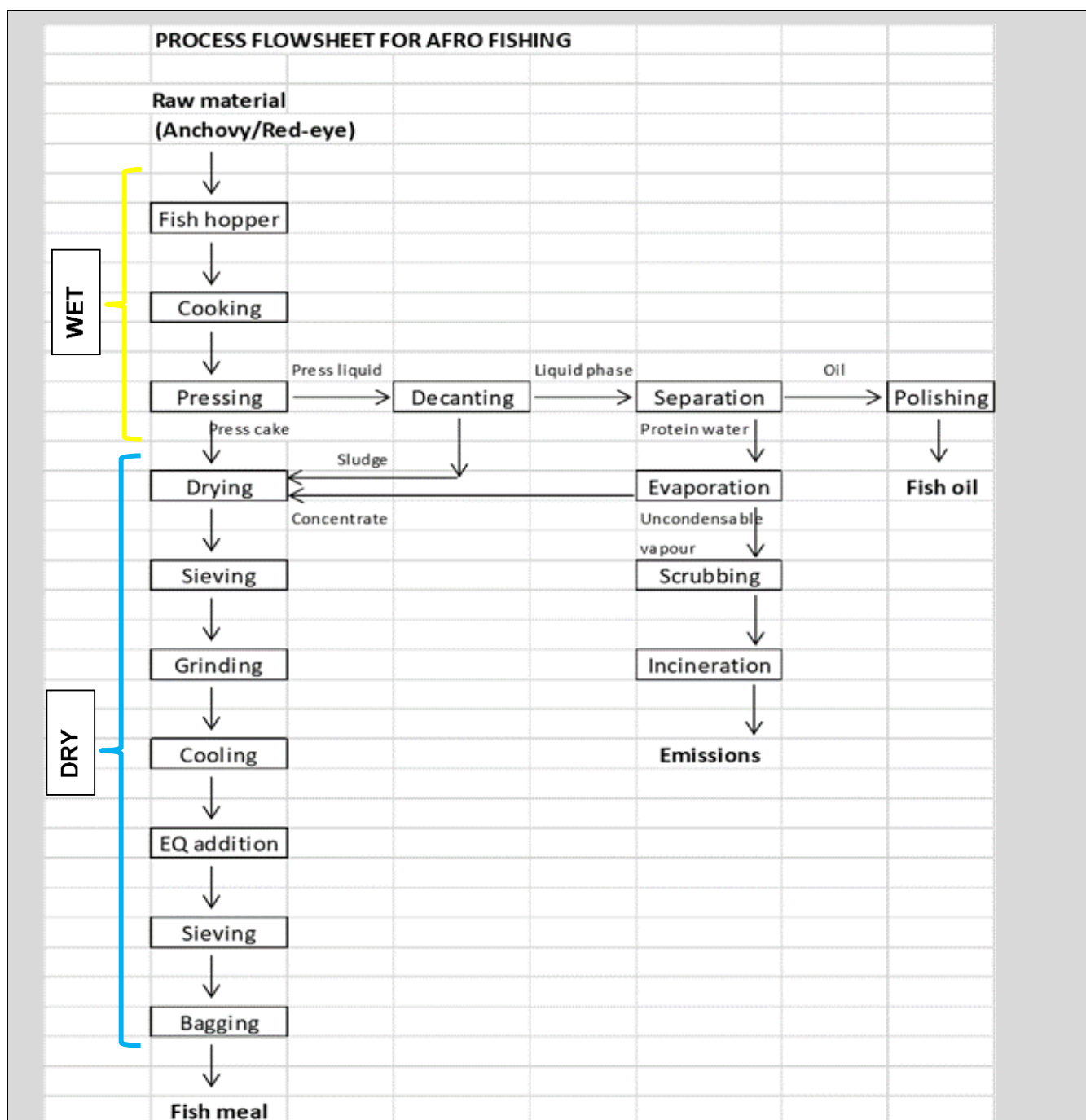
Figure 23: Process Flow Chart
