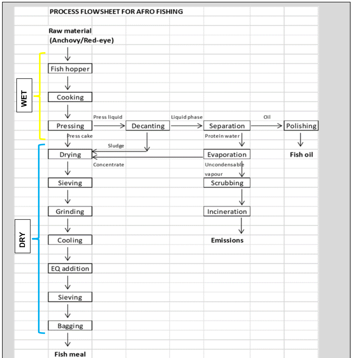
Figure 14: Process Flow Chart
