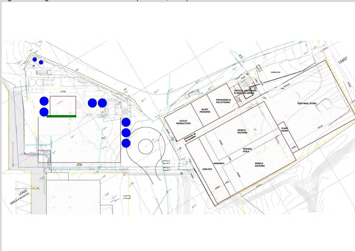
Figure 46: Proposed expansion layout
