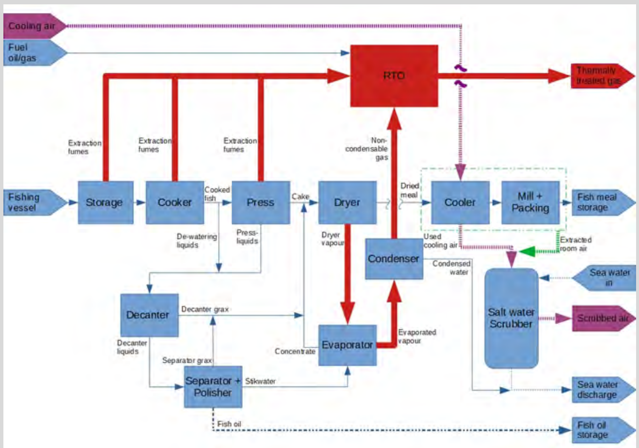
Figure 49: Process Flow Diagram (LAQS, 2019)
